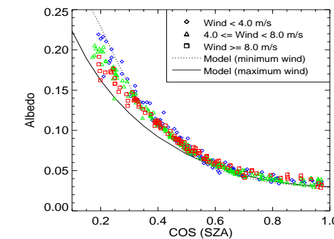
Fig. 6. Wind effects on ocean surface albedo. The observed albedo as a function of the cosine of SZA are plotted in three wind categories. The dashed line and the solid line are the modeled albedo with the minimum wind (0.48 m/s) and maximum wind (14.0 m/s) of the observations, respectively. The mean AOD and PW of measurements were used in model calculations.
